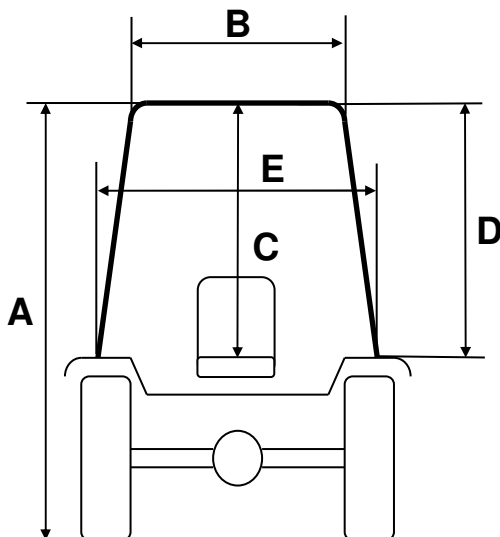
Cabina PASQUALI Eos L65 RS Monodirectional Tractor Tyres 280/70 R.18
