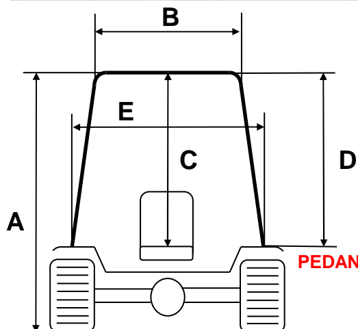
CABINA SAME KRYPTON "F" 100 Stage III B
