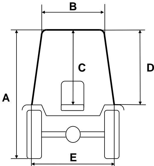
CABIN CARRARO Tractors AGRICUBE FB115 Back Tyres 380/70 R.24
