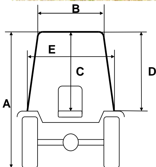
CABIN SAME KRYPTON3 80 V Euro III
